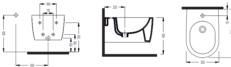
W.HUNG BIDET 52 CM SINGLE HOLE SOBA05201VD1W5000 520x355 mm
