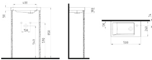
INFINITIUM VANITY WB. 50 CM SINGLE HOLE INLK05001FD1W5000 500mm
