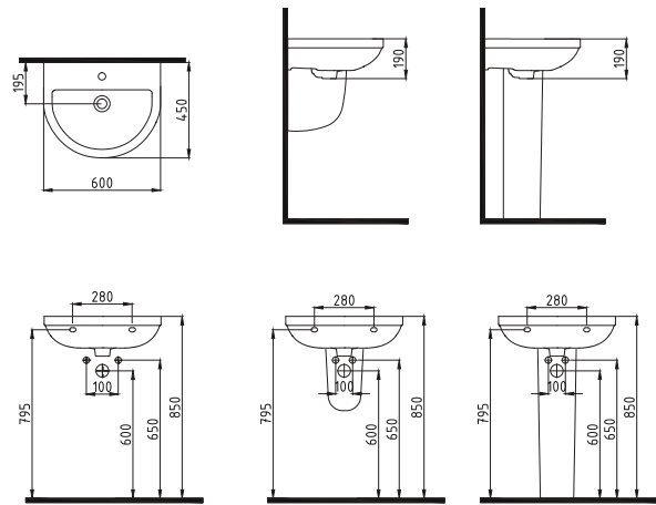
CAPRI WB. WALL MOUNTING OPTION 60 cm SINGLE HOLE WHITE CPLS060B1VD1W5000 600x450 mm
