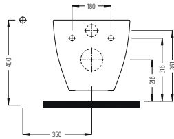
WALL HANG WC PAN 52 CM NO-RIM NCKA052N2VP1W5000 520x355 mm
