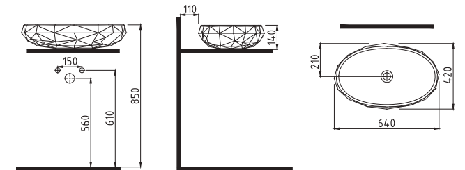
COUNTERTOP WASHBASIN 62 cm WITHOUT HOLE MLLG06201FDOW5000 640x420mm
