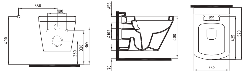
NEPTUN WALL HUNG WC PAN 52 cm NPKA052AMVPOW5000 520x350mm
