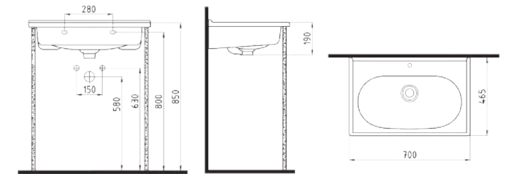
VANITY WASHBASIN 70 cm SINGLE HOLE FELK070B1FD1W5000 700x465mm
