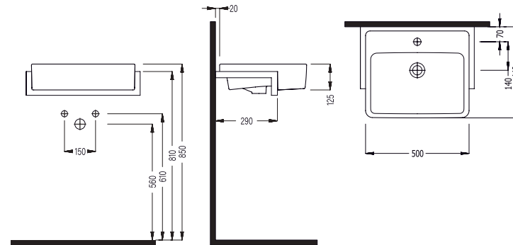
RECTANGLE SEMI RECESSED WB. 50 CM SINGLE HOLE ROLY05003FD1W5000 500x440 mm
