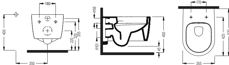
W. HUNG WC PAN 52 CM NO-RIM WITHOUT BIDET FUNCTION SOKA052N1VPOW5000 520x355 mm
