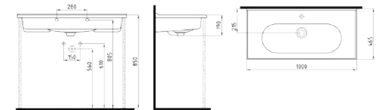
VANITY WASHBASIN 100 cm SINGLE HOLE FELK10001FD1W5000 1000x465mm
