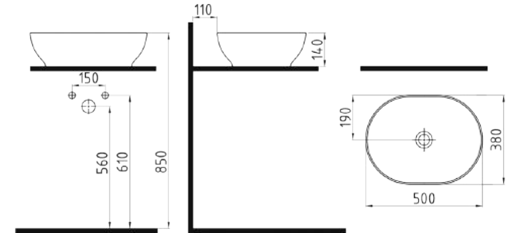
OBLONG COUNTERTOP WASHBASIN 50 cm WITHOUT HOLE MTLG05001FDOW5000 500x380mm
