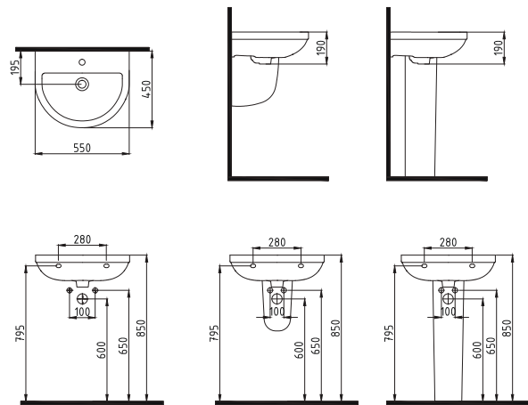
CAPRI WB. WALL MOUNTING OPTION 55 cm SINGLE HOLE WHITE CPLS055B1VD1W5000 550x450 mm
