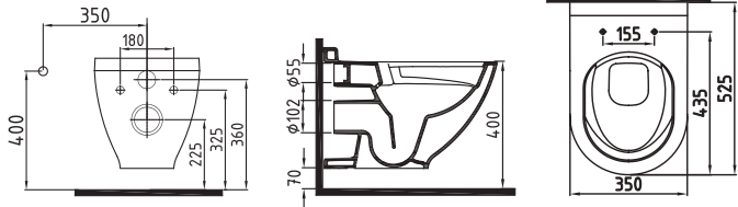
WALL HUNG WC PAN 52 CM NO-RIM CONCEA- LED FIXING HRKA052N5VP0W5000 520x350mm
