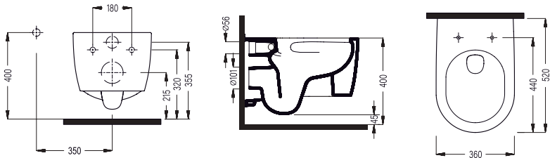
WALL HANG WC PAN 52 cm SOFTFLUSH CONCEALED FIXING (VORTEX FLUSHING SYSTEM) SOKA052VIP1W5000 520x360 mm
