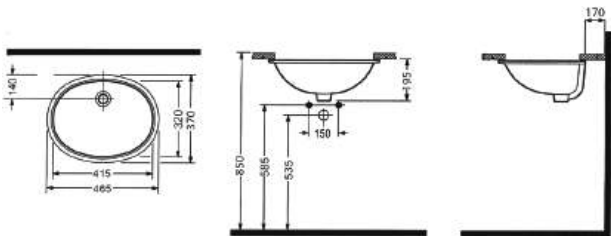
SINGLE PIECE UNDERCOUNTER WASHBASIN 41 cm WITHOUT HOLE TPLA04101VDOW5000
