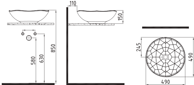
COUNTERTOP WASHBASIN 49 cm WITHOUT HOLE PNLG04901FD0W5000 Ø490mm
