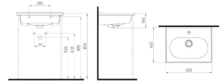
VANITY WASHBASIN 60 cm SINGLE HOLE FELK060B1FD1W5000 600x465mm
