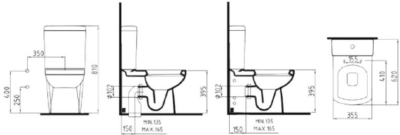
BACK TO WALL CLOSE COUPLED WC PAN 62 cm GYKD06201VPOW5000 620mm
