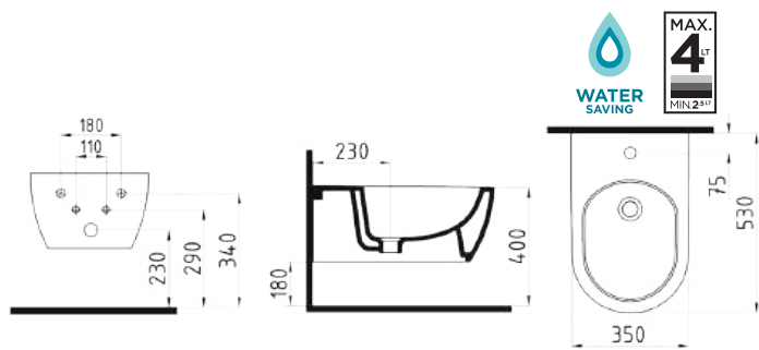
WALL HUNG BIDET 52 cm N3 SINGLE HOLE HRBA05203VD1W5000 530x350mm
