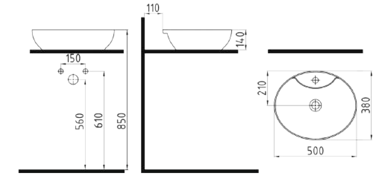
OVAL COUNTERTOP WASHBASIN 50 cm WITH HOLE MTLG05005FD1W5000 500x380mm
