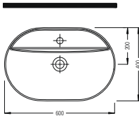
OBLONG COUNTERTOP WASHBASIN 60 cm SINGLE HOLE NCLG06001FD1W5000 600x400 mm
