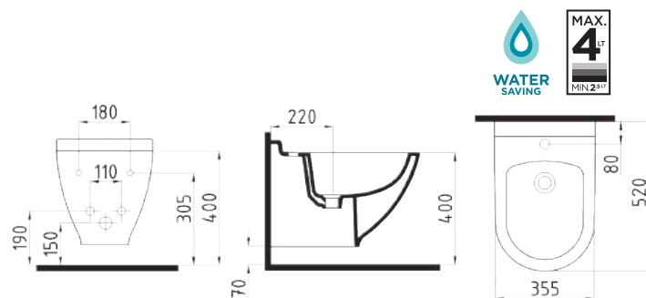
WALL HUNG BIDET 52 cm CONCEALED FIXING SINGLE HOLE HRBA05201VD1W5000 520x350mm
