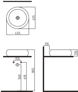
COUNTERTOP WASHBASIN 46 cm WITHOUT HOLE SATIN PLATIN COATED FALG04601FD0X8SZ0 Ø 460mm
