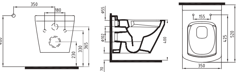
NEPTUN WALL HUNG WC PAN 52 cm NO-RIM CONCEALED FIXING NPKA052N1VPOW5000 520x350mm
