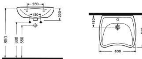
SINGLE PIECE DISABLED WASHBASIN 60 cm SINGLE HOLE TPLE06001VD1W5000 600x510mm
