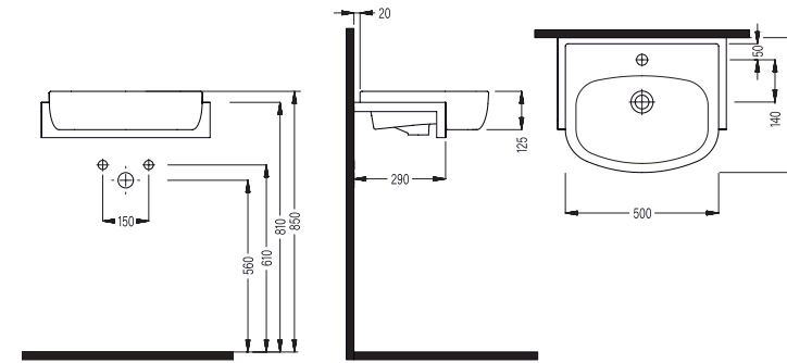
SEMI RECESSED WB. 50 CM SINGLE HOLE ROLY05001FD1W5000 500x440 mm
