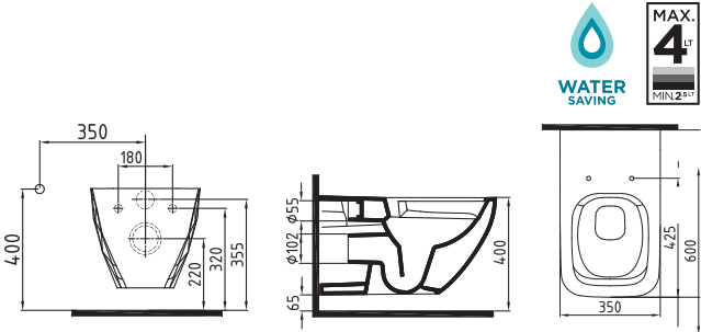
WALL HUNG WC PAN 60 cm NO-RIM/ CONCEALED FIXING KRKA060N1VP0W5000 600x350mm White
