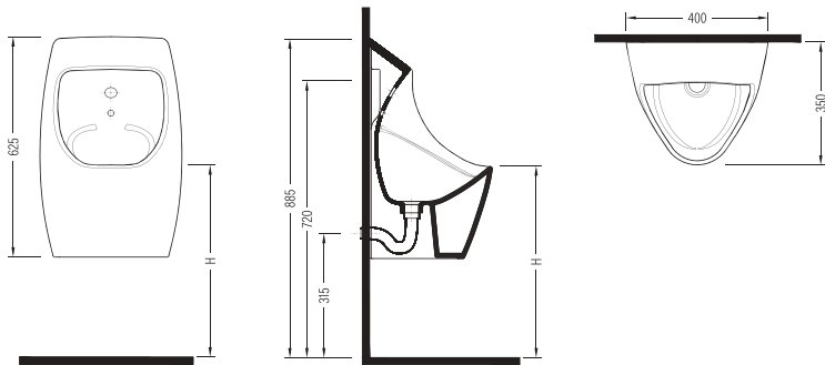
HARMONY URINAL 62 cm REAR INLET WITH PHOTOCELL BATTERY/ ELECTRIC COOL WHITE EXT. HRPS06205VSAW5000
