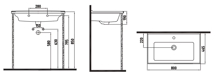
VANITY WASHBASIN 80 cm SINGLE HOLE NPLK080B1FD1W5000 800x470mm
