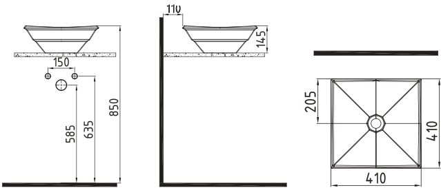
COUNTERTOP WASHBASIN 41 cm WITHOUT HOLE KRLG04101FDOW5000 410x410mm White
