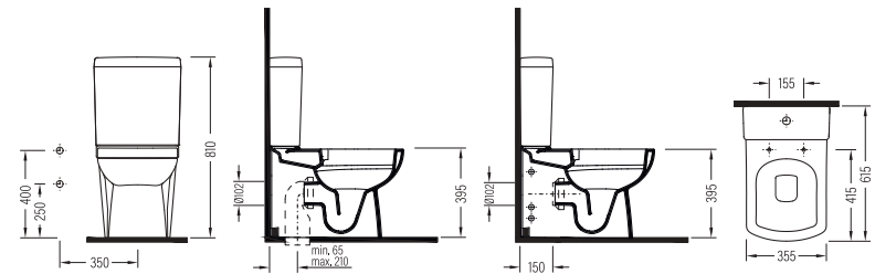
BACK TO WALL CLOSE COUPLED WC PAN 62 CM NO-RIM GYKD062N1VPOW5000
