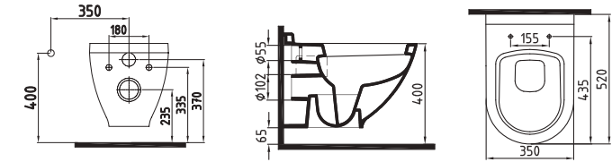
WALL HUNG WC PAN 52 cm HRKA052AMVP0W5000 520x350mm
