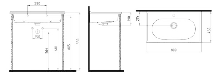
VANITY WASHBASIN 80 cm SINGLE HOLE FELK080B1FD1W5000 800x465mm
