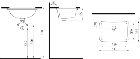
SINGLE PIECE UNDERCOUNTER WASHBASIN 45 cm WITHOUT HOLE TPLA04501VDOW5000
