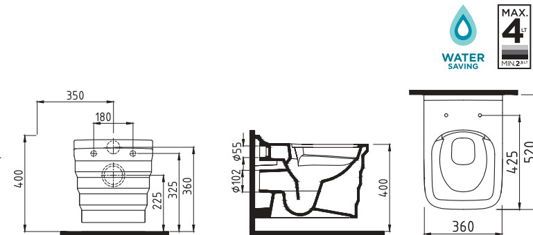
WALL HUNG WC PAN 52 cm NO-RIM/ CONCEALED FIXING SHKA052N1VPOW5000 520x360mm
